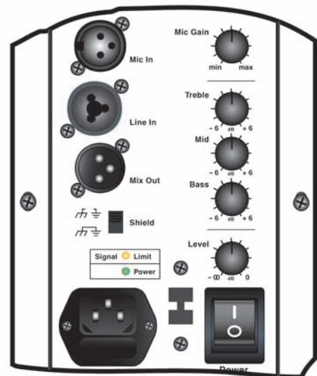
YX15P Rear Panel
