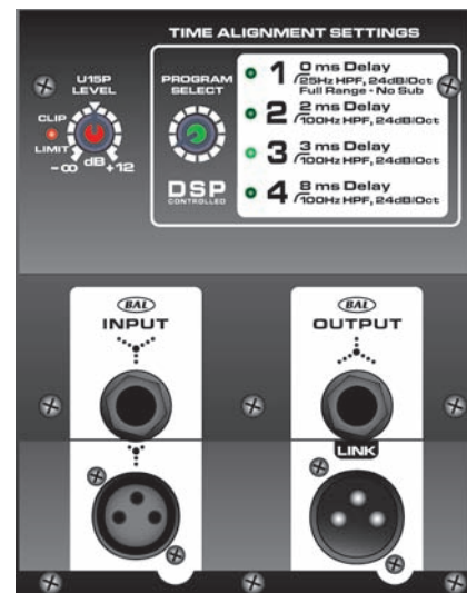
U15P Rear Panel
