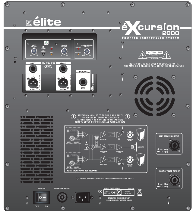
EX2 Rear Panel
