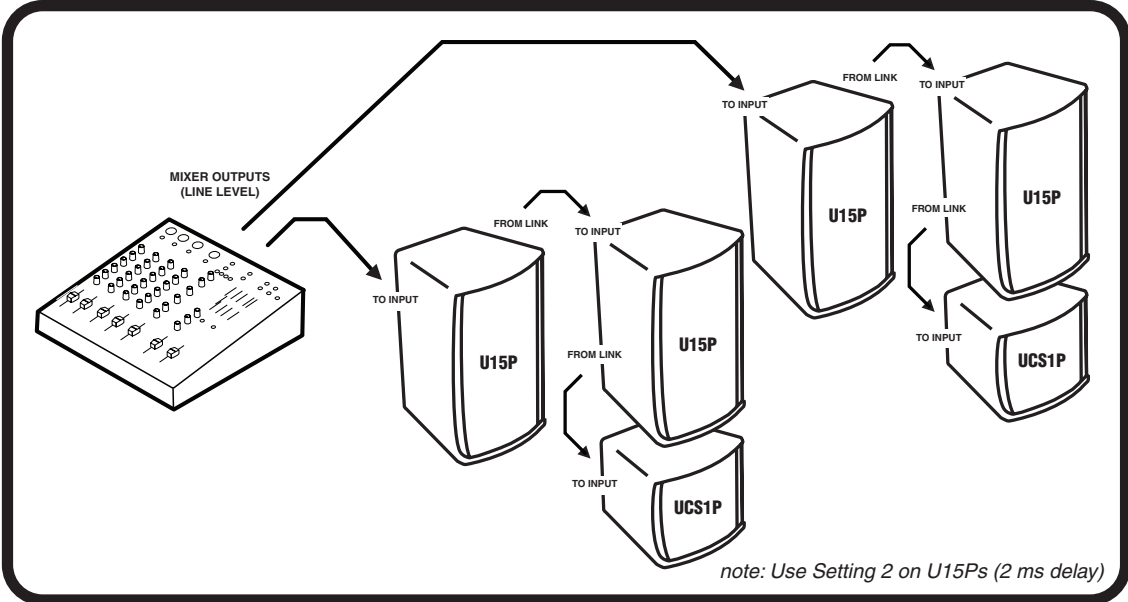
STEREO P.A., using a MIXER, DUAL U15Ps/Ch. and SUBWOOFERS
