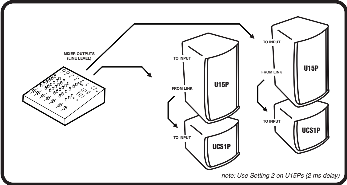
STEREO P.A., using a MIXER, MULTIPLE U15Ps and SUBWOOFERS
