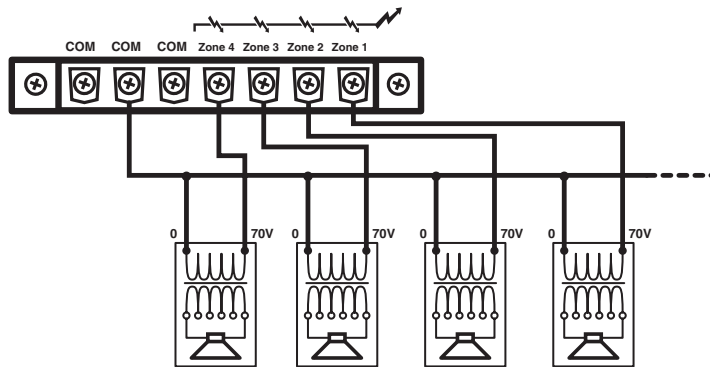
Connecting the speakers to 70V output
